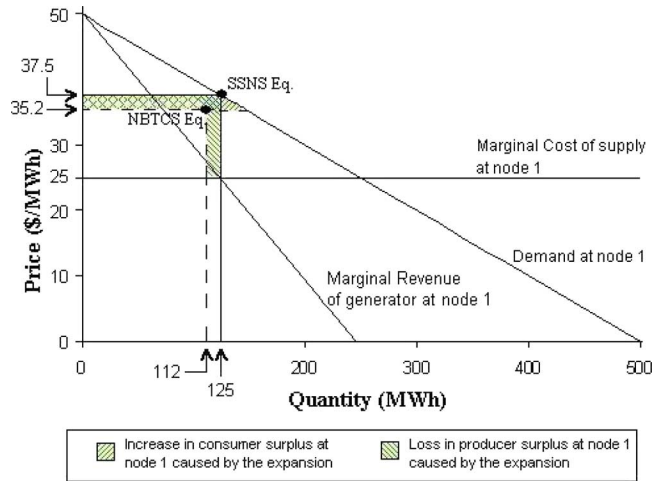
Fig. 2. Equilibrium at node 1 under both the SSNS and the NBTCS.
